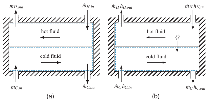
Figure 4-11: (a) Mass balances and (b) energy balances on each side of a heat exchanger.
