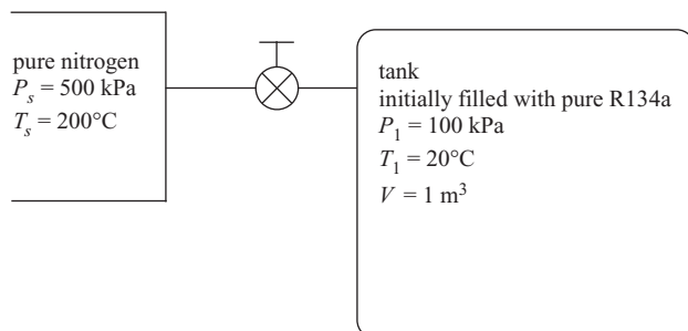
Figure 12.A-13: Tank containing refrigerant vapor connected to a source of nitrogen.
