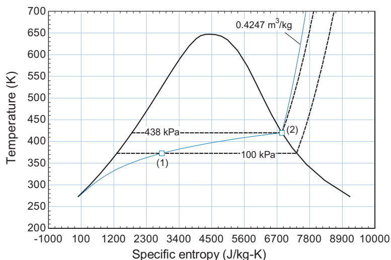
Figure 3: Temperature–specific entropy plot for the water heating process.
