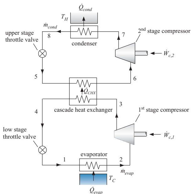
Figure 1: Cascade system.
