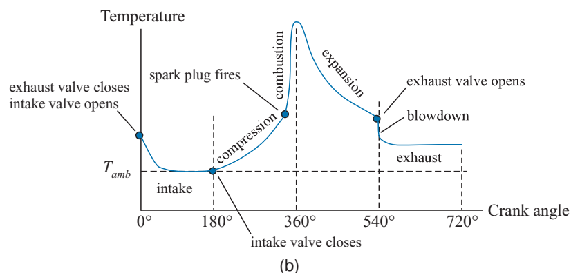
Figure 8-33: (a) Pressure and (b) temperature of the gas in the cylinder shown qualitatively as a function of crank angle.
