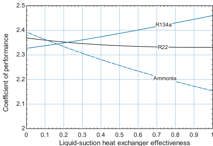
Figure 1: COP as a function of the liquid-suction heat exchanger effectiveness.
