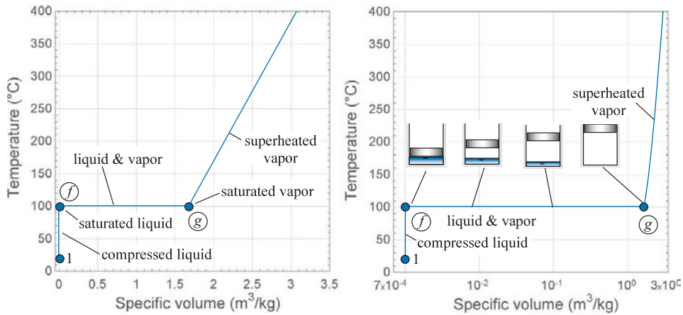
Figure 2-5: Temperature as a function of specific volume for water at 101.3 kPa using (a) a linear and (b) a logarithmic scale for specific volume.
