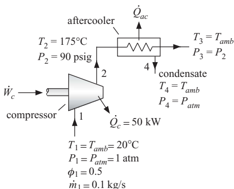
Figure 12.A-3: Air compressor with aftercooler.
