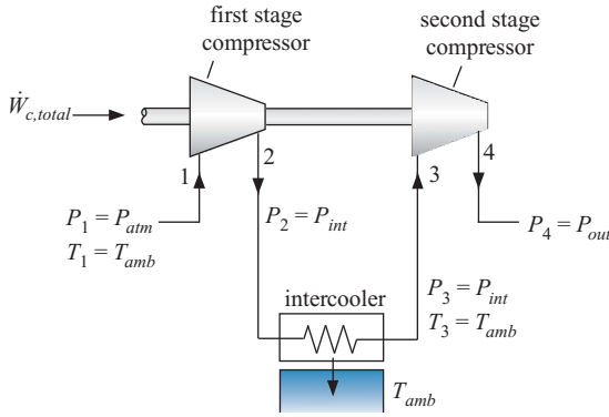
Figure 1: Two-stage, intercooled compressor.
