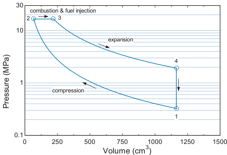
Figure 2: Pressure-volume diagram for Diesel cycle.
