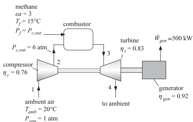
Figure 1: Gas turbine engine.
