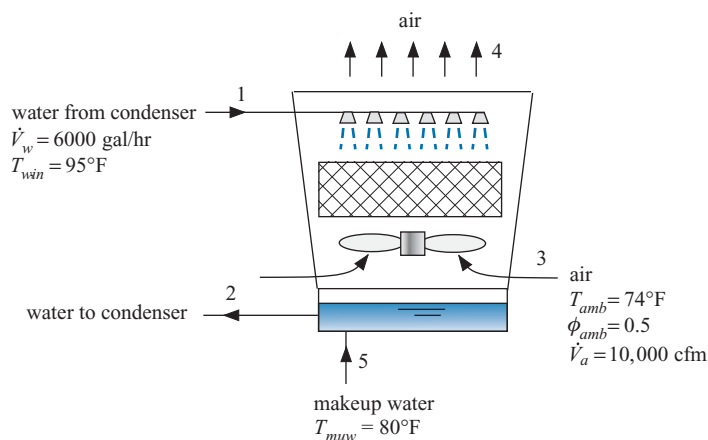
Figure 1: Cooling tower.
