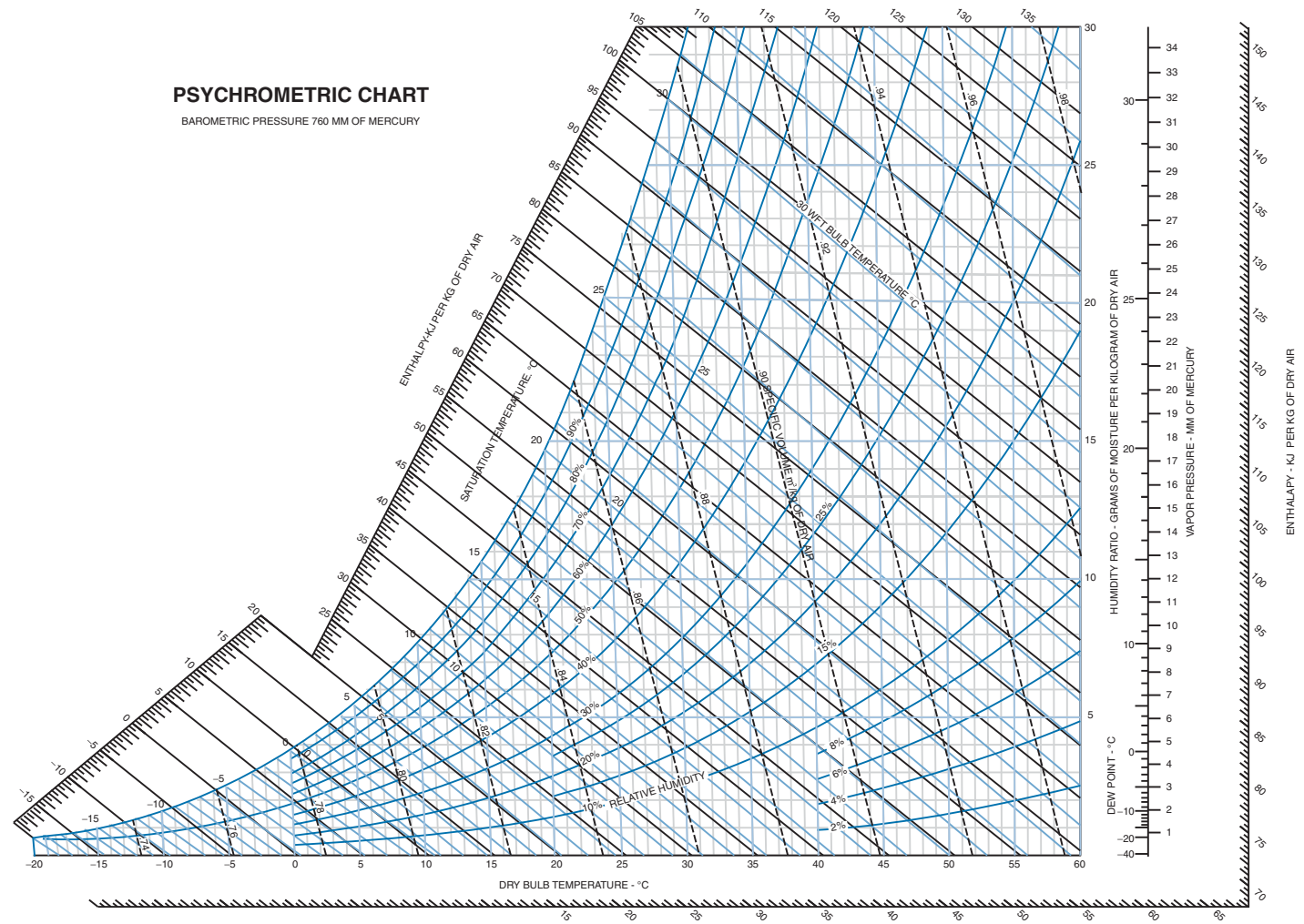
Figure 12-6: Psychrometric chart in SI units for P = 101.3 kPa. (From Universal Industrial Gases Inc., http://www.ugi.com/UIGI_SI.PDF with permission)
