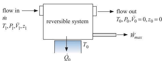
Figure 7-3: Flow stream at state 1 entering a steady-state, reversible system that interacts with the environment at the dead state and will therefore produce the maximum possible power.
