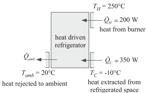
Figure 6.A-29: Heat-driven refrigerator.
