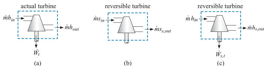
Figure 6-10: (a) An energy balance on the actual turbine and (b) an entropy balance and (c) an energy balance on the reversible turbine that is used to bound the performance.
