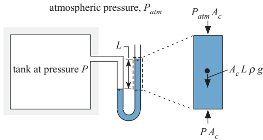
Figure 1-7: Manometer.
