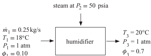
Figure 12.A-2: Humidifier.
