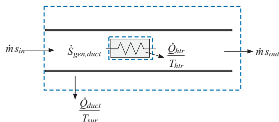
Figure 4: Entropy balance on duct, excluding the heater.
