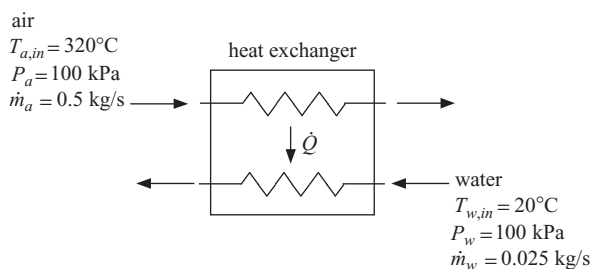
Figure 6.B-2 Heat exchanger.
