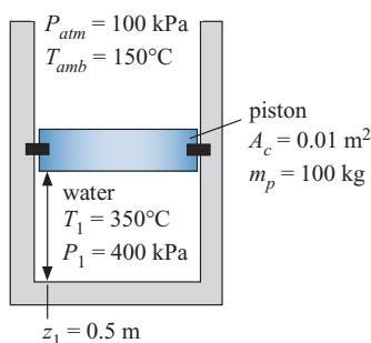
Figure 6.A-31: Piston-cylinder device.
