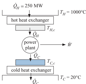
Figure 6.A-5: Power plant.
