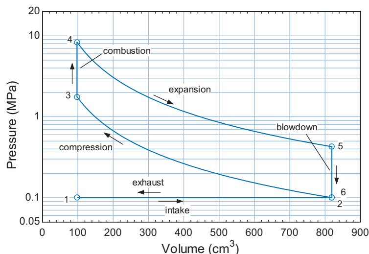
Figure 1: Pressure-volume diagram.
