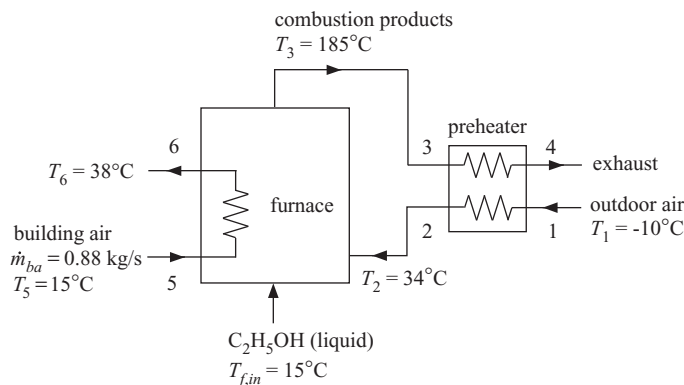
Figure 13.B-22: Furnace with preheater that uses ethanol as the fuel.
