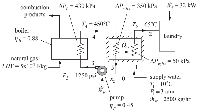
Figure 1: Boiler providing hot water to a commercial laundry.
