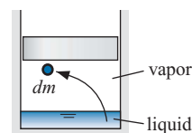
Figure 10-14: Two phase liquid-vapor system at equilibrium showing a small mass moving from liquid to vapor phase.
