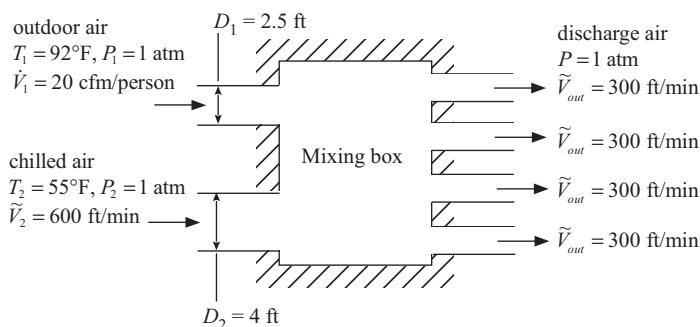
Figure 4.A-1: Mixing box.
