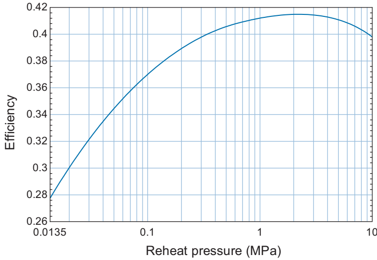
Figure 8-14: Efficiency of the ideal Rankine cycle with reheat as a function of the reheat pressure. The cycle is operating with water with T_H = 800 K, T_C = 325 K, and P_b = 10 MPa.
