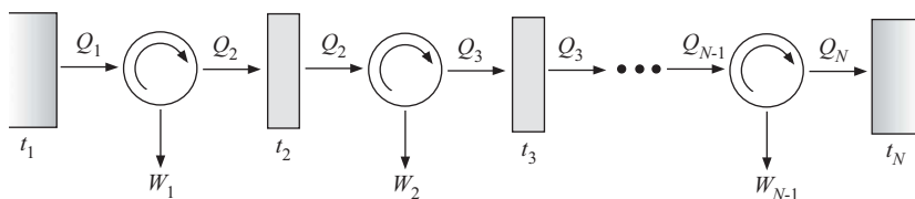
Figure 3: Series of reversible heat engines operating between temperature t_i and t_N , the temperature of each subsequent temperature reservoir decreases by t_i - t_{i+1} = 1^\circ\text{S} where t is a new temperature scale that is defined so that the efficiency of each engine is identical.
