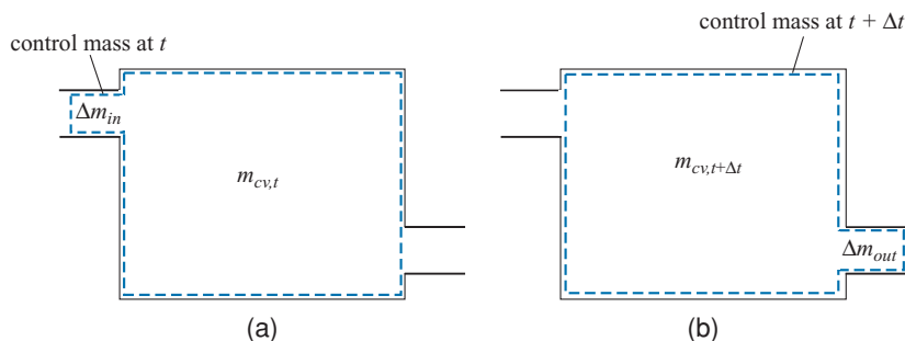
Figure 4-2: Closed system enclosing a fixed amount of mass (a) at time t , and (b) at time t + \Delta t .
