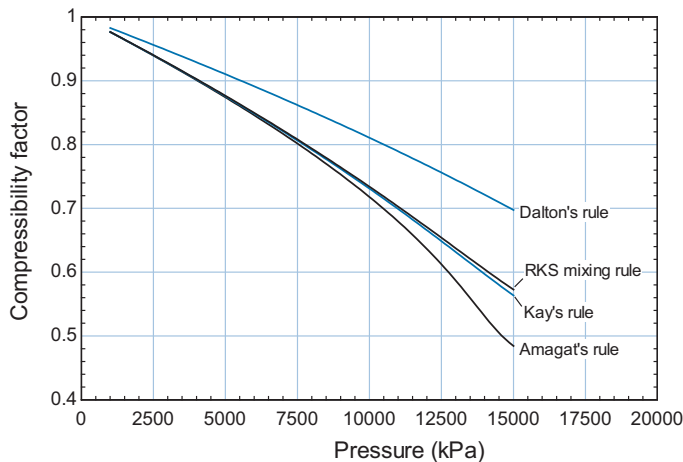
Figure 1: Compressibility factors predicted using Dalton’s rule, Amagat’s rule, Kay’s rule, and the RKS mixing rule as a function of pressure for a mixture that is 20% \text{CO}_2 and 80% ammonia (by mole) at 150^\circ \text{C} .
