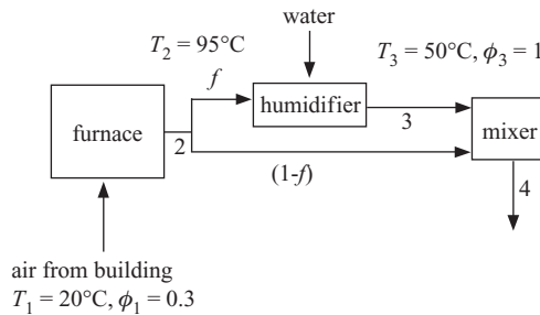
Figure 12.B-2: Humidifier.
