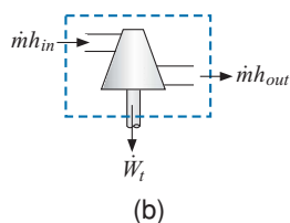
Figure 4-6: (a) Schematic of an axial turbine and (b) the symbol for the turbine component.
