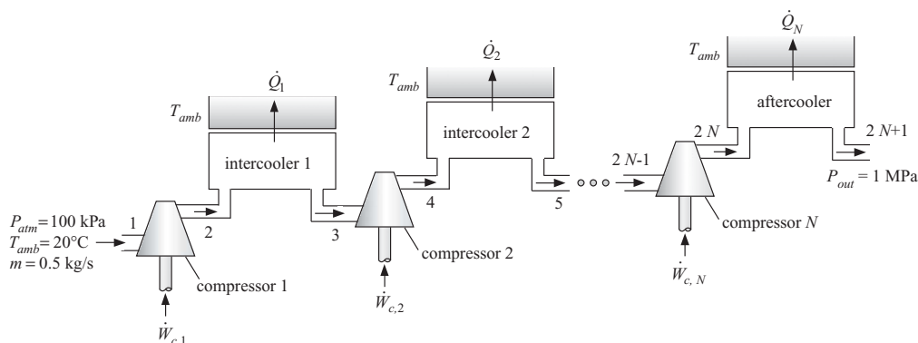
Figure 5: Intercooled compression process.
