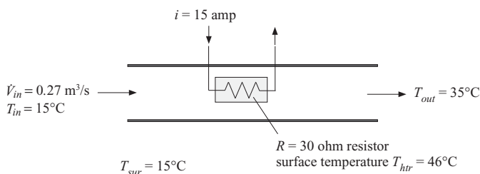
Figure 1: Air heating system.
