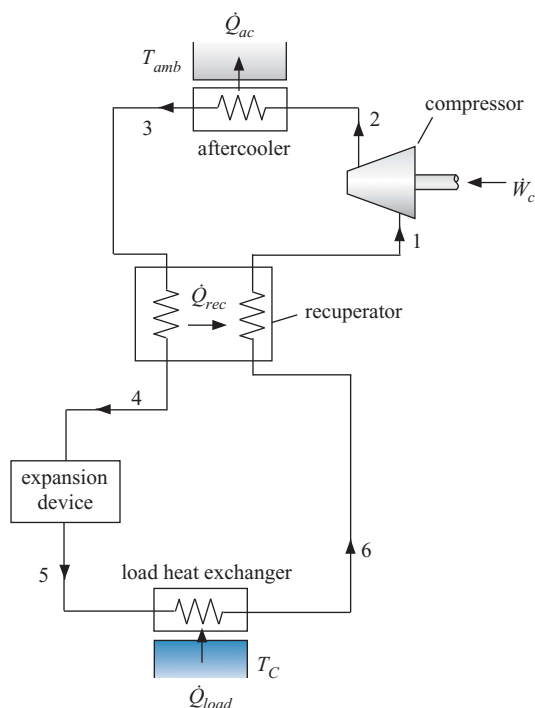
Figure 9-25: Basic recuperative cooling cycle.
