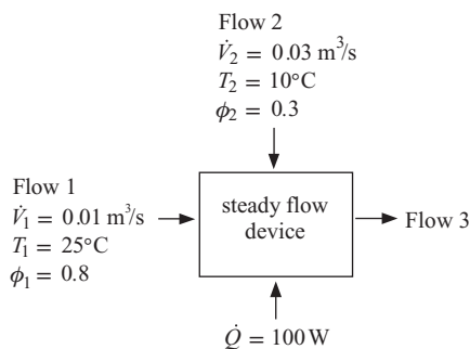
Figure 12.A-5: Steady flow device.
