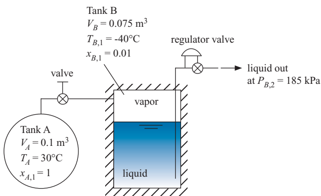
Figure 4.B-9: Liquid transfer equipment.
