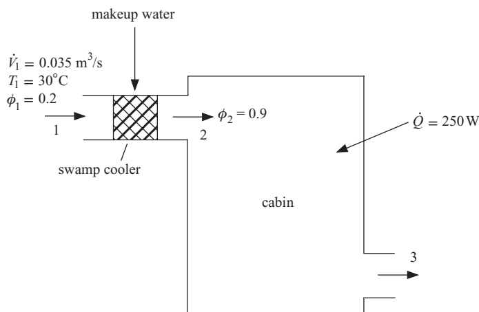
Figure 12.B-3: Swamp cooler.
