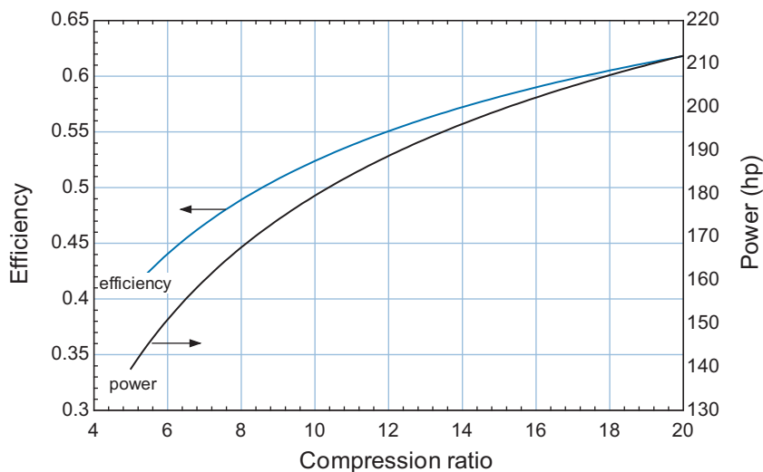
Figure 8-36: Power and efficiency as a function of compression ratio.
