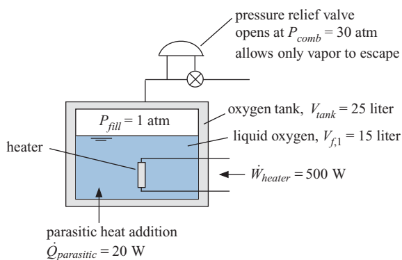
Figure 4.B-3: Oxygen tank.
