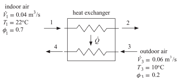
Figure 12.A-4: Heat exchanger.
