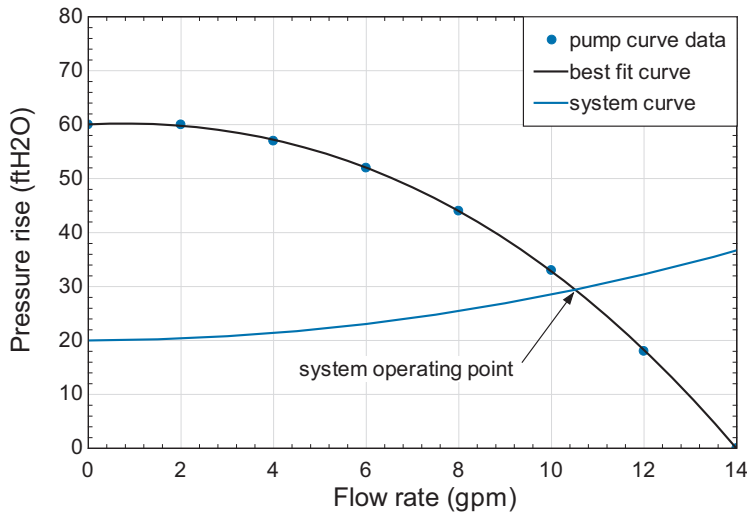
Figure 3: Pump curve data with best fit curve and system resistance curve. The intersection is the operating point.
