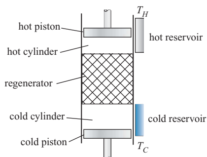
Figure 8-42: The Stirling engine.
