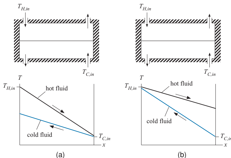
Figure 6-23: Counterflow exchanger operating with constant specific heat capacities where (a) \dot{C}_H < \dot{C}_C so the pinch point occurs at the cold end, and (b) \dot{C}_C < \dot{C}_H so the pinch point occurs at the hot end.
